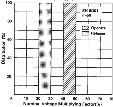
Distribution of Operate & Release Voltage (DC Type)
