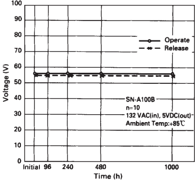
High temperature Continuous Operating Test (AC Type)
