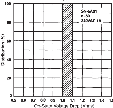
Distribution of On-State Voltage Drop (AC Type)
